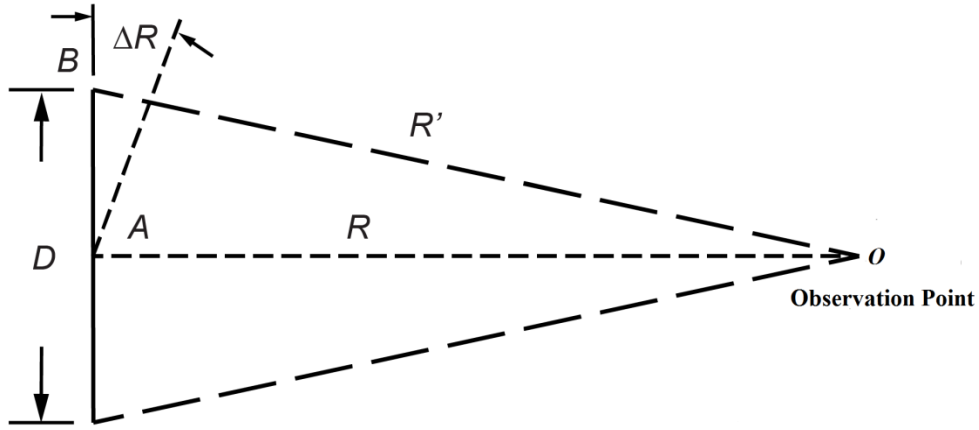
Figure 2 Derivation of Fresnel-Fraunhofer Boundary Sphere
