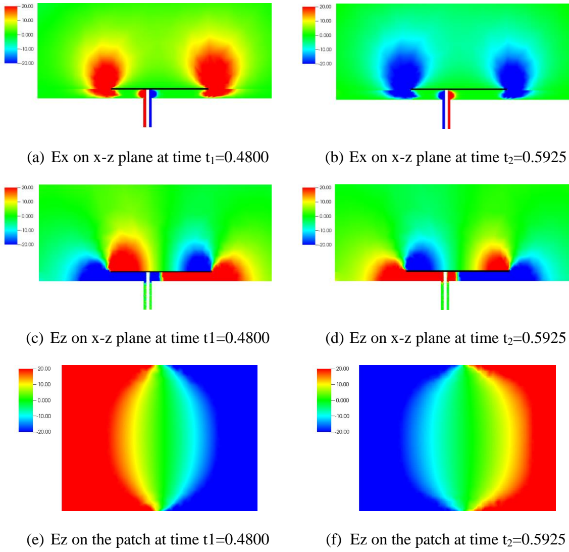
Figure 29 Electric Fields of Patch Antenna on x-z Plane and Patch
