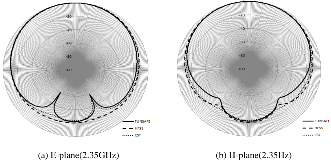
Figure 36 Comparison of Radiation Pattern at 2.35GHz Calculated by HFSS,CST and FUNSAFE on Fine Mesh with Hemispherical Computational Domain with the P2 Scheme in the Case of Patch Antenna ( \epsilon_r = 2.2 )
