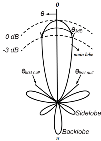
Figure 1 Antenna Pattern in Plane \varphi = \text{const.}
