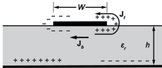
Figure 25 Current Distribution of Cavity Model
