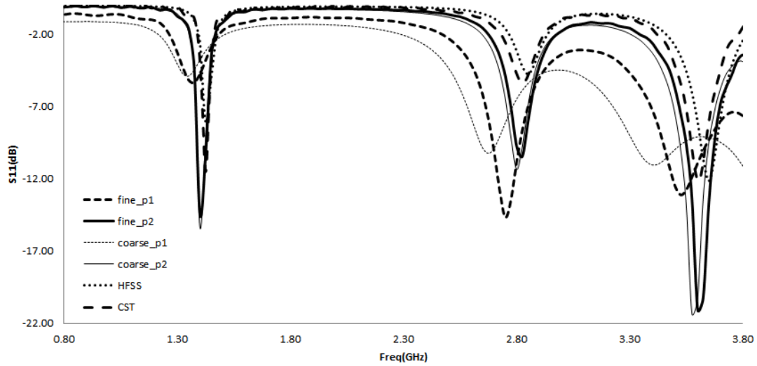
Figure 35 Comparison of S_{11} Calculated by HFSS, CST and FUNSAFE on Different Meshes with P1 and P2 Schemes in the Case of Patch Antenna ( \epsilon_r = 6.6 )
