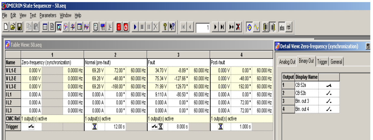
Figure 4.5: Four states selected for testing the line
