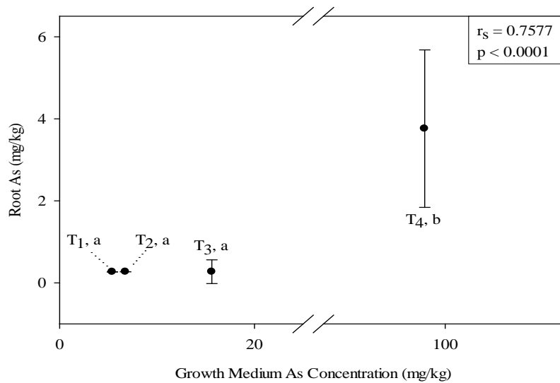
Figure 3 Median ( \pm IQR) As concentrations of the root portion of sampled beets as a function of As concentrations in growth medium. Medians denoted by the same letter indicate no significance (Fischer's LSD, \alpha = 0.05 ). See Table 3 for concentrations of As in each treatment.
