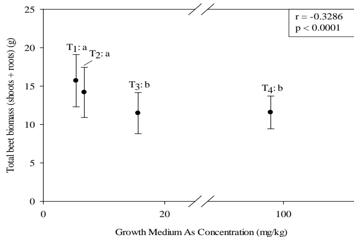
Figure 2 Mean biomass production (g) of sampled beets as a function of growing medium As concentration (mg/kg). Means denoted by the same letter indicate no significance (Tukey-Kramer, \alpha = 0.05 ). A marked decrease in biomass production between T 2 and T 3 indicate a potential threshold of phytotoxicity. See Table 3 for concentrations of As in each treatment.
