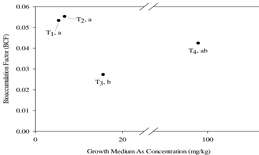
Figure 5 Bioaccumulation Factor (BCF). BCF is a standardized dimensionless value that represents the potential for an organism to accumulate toxins from its surroundings (Branson et al. 1975). Higher BCF values indicate that a higher proportion of available As was accumulated into the tissues of the beets for that treatment. BCF values denoted by the same letter are not significantly different ( \alpha = 0.05 ). See Table 3 for specific values.
