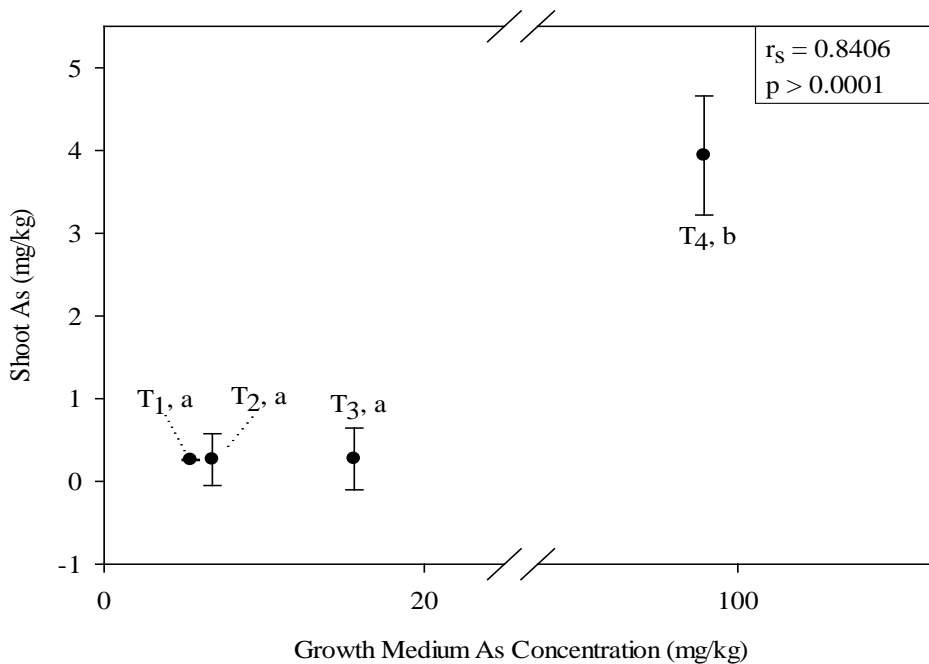
Figure 4 Median ( \pm IQR) As concentrations of the shoot portion of sampled beets as a function of As concentrations in growing medium. Medians denoted by the same letter indicate no significance (Fischer's LSD, \alpha = 0.05 ). See Table 3 for specific values.
