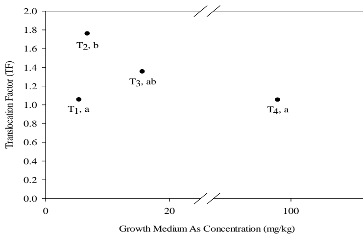
Figure 6 Translocation Factor (TF) as a function of growing medium As concentration. TF is a dimensionless value that is a measure of the tendency for a plant to translocate a toxicant from the subterranean portion to the above ground portion of the plant. A value of < 1 indicates that more of the toxicant (in this case As) remains in the subterranean tissues. A value that is > 1 indicates that the plant tends to translocate the toxicant to the above ground portion, and a value of 1 indicates that there is no preference by the plant (Singh & Agrawal 2007). TF values denoted with the same letter are not significant ( \alpha = 0.05 ). See Table 3 for specific values.
