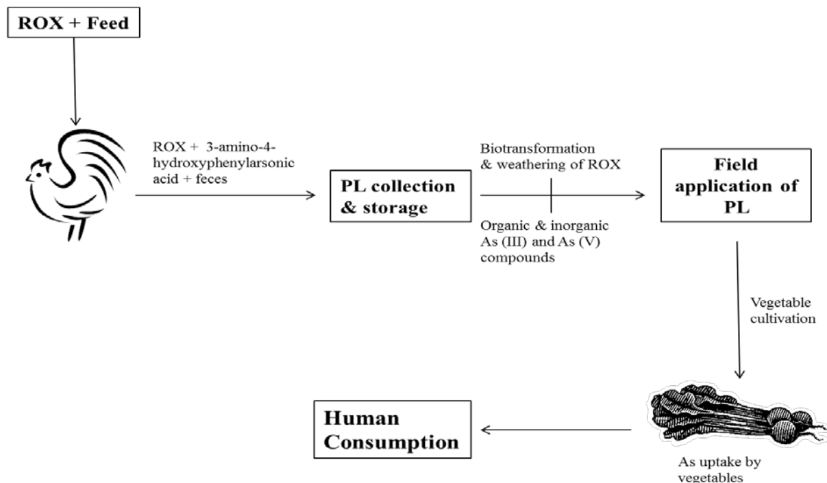
Figure 1 Potential pathway from ROX administration to poultry, deposition into poultry litter (PL) (Moody & Williams 1964), biotransformation of ROX into more mobile As species, application to agricultural fields (Kpombrekou et al. 2002, Garbarino et al. 2003), uptake of As by food crops (Wang et al. 2006), and subsequent human exposure.
