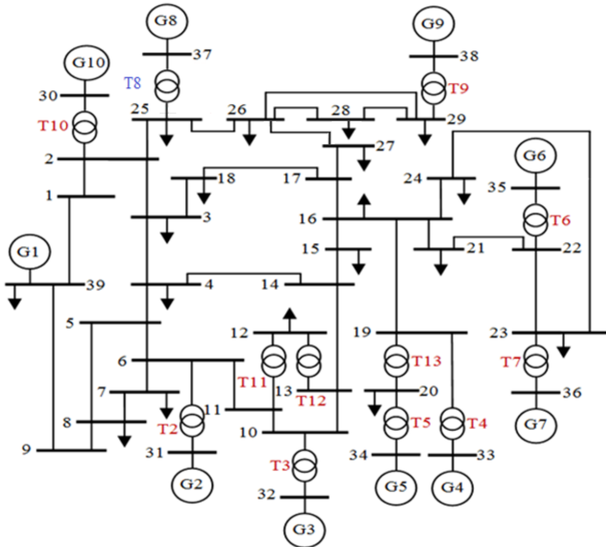
Figure 4.1 IEEE39-bus system
