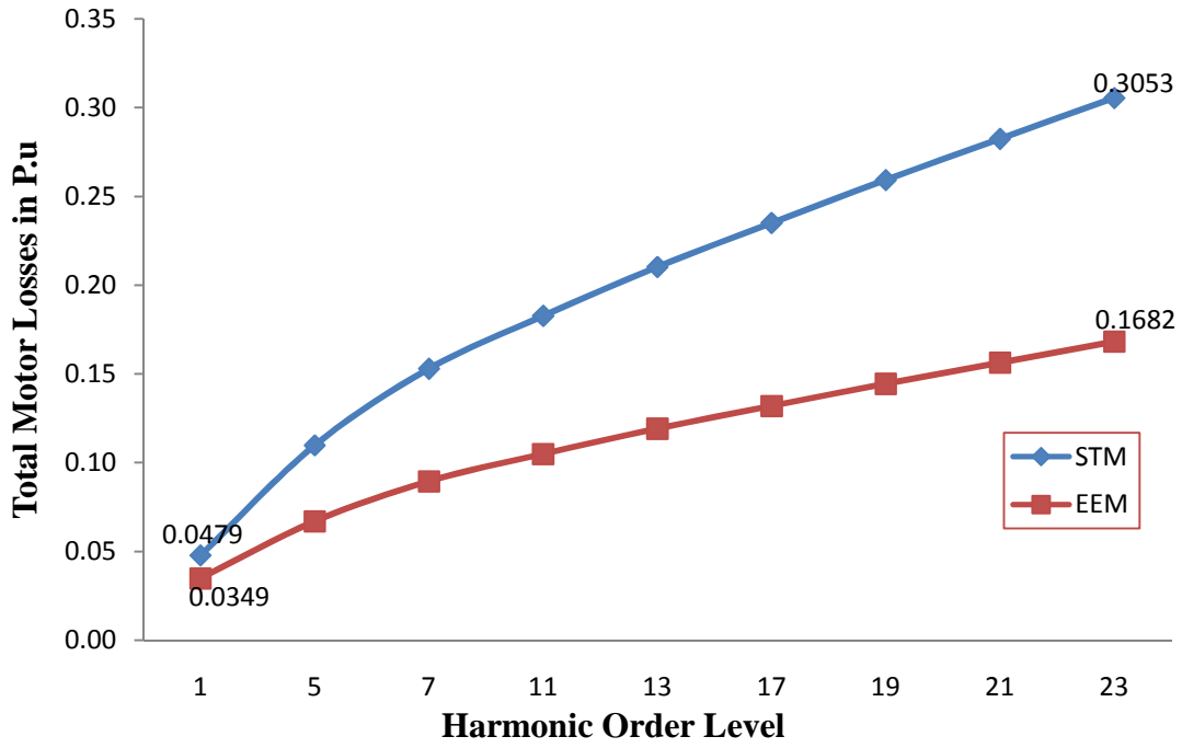
Figure 4.41: Cumulative Total Losses for 200HP Motors
