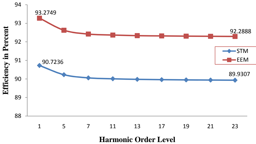
Figure 4.6: Efficiencies for 25 HP Motors vs. Harmonic Order Level
