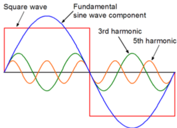
Figure 3.3: Harmonic Waveform
