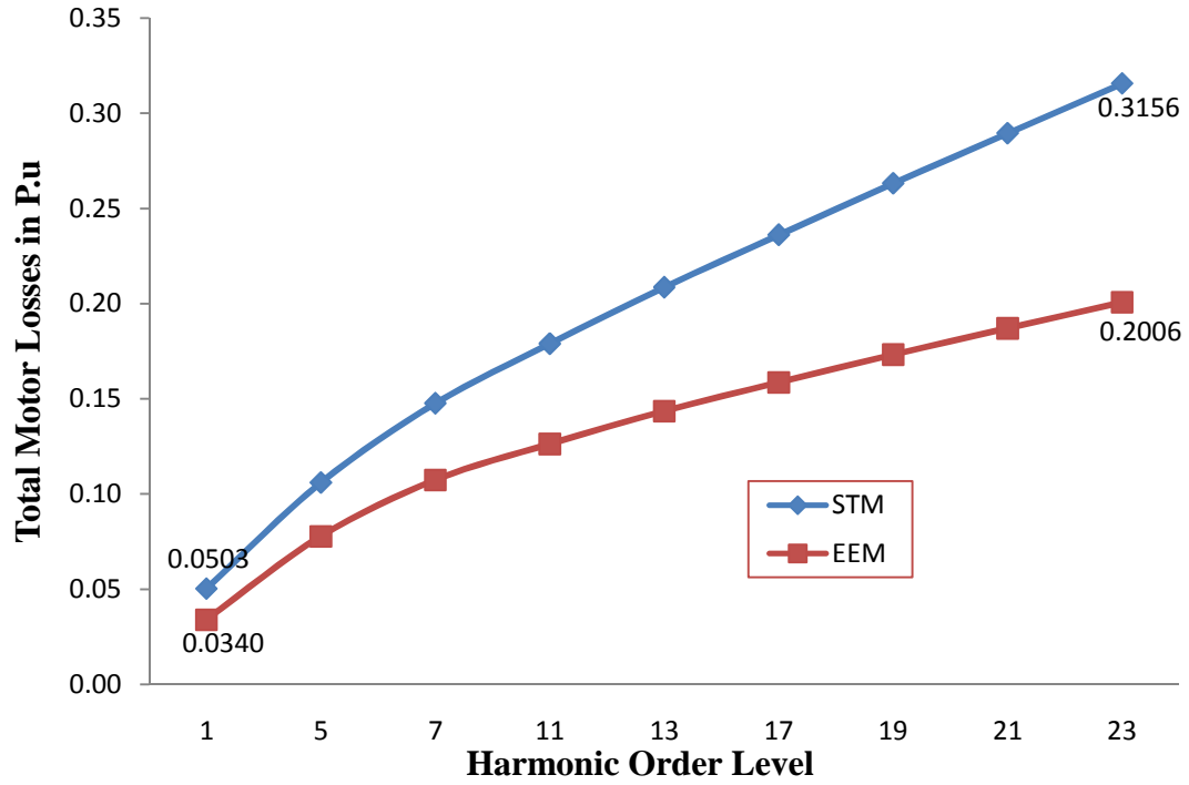
Figure 4.51: Cumulative Total Losses for 250HP Motors
